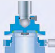
Conversion kit for balanced bellows See Art.-No. page 01/79
