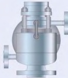
Balanced bellows J83: Bellows INCONEL J78: Bellows 1.4571 J88: High temperature equipment
