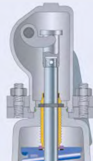
Bolted lifting device H6 K06
