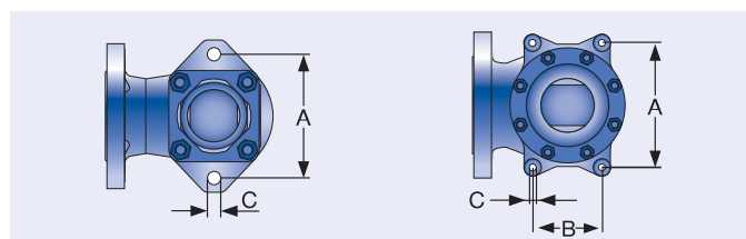
Support brackets
