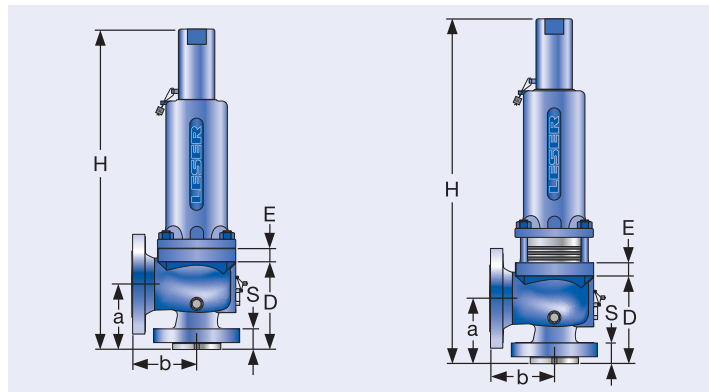
Conventional design
